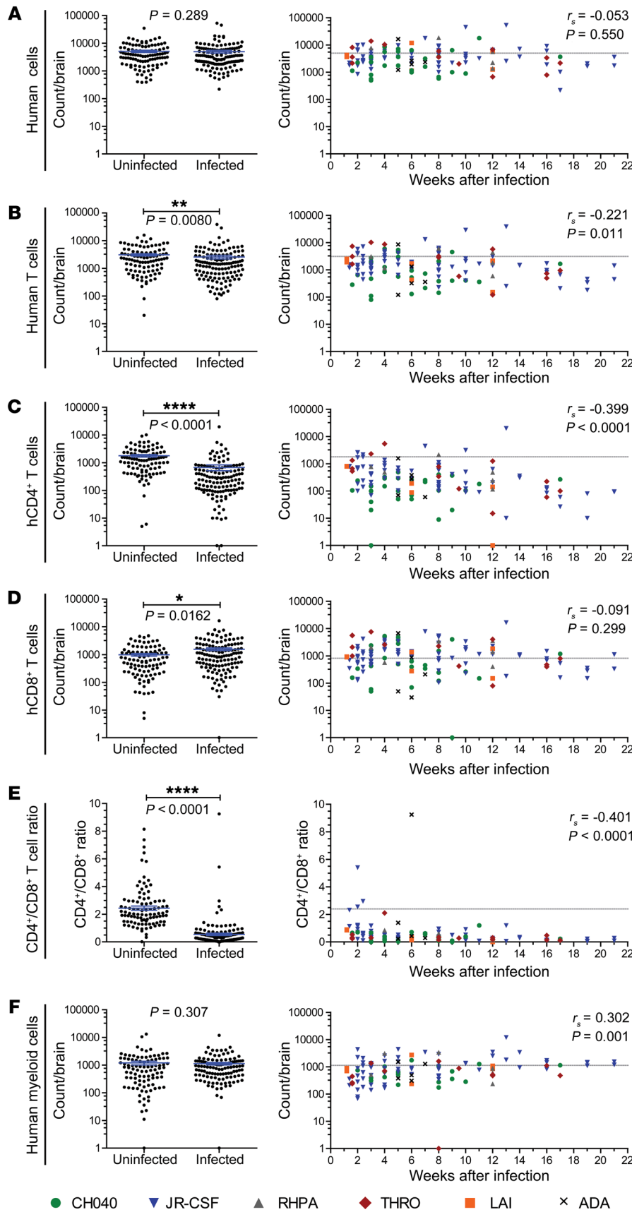
Figure 5. Alterations in human T cell populations in the brains of HIV-infected BLT mice. Total numbers of human (A) hematopoietic cells (hCD45 + ), (B) T cells, (C) CD4 + T cells, (D) CD8 + T cells, (E) the CD4 + /CD8 + T cell ratio, and the numbers of (F) myeloid cells in the brains of HIV-infected ( n = 132 ) or uninfected ( n = 104 , from Figure 3) BLT mice were determined by flow cytometry. Left panels indicate the absolute number of cells or CD4 + /CD8 + T cell ratio in the brains of uninfected and HIV-infected BLT mice. Right panels indicate the absolute number of cells or CD4 + /CD8 + T cell ratio in the brains of HIV-infected BLT mice and the time points after infection at which analysis was done. Mice infected with the same HIV strain are shown with the same color and symbol (CH040: green circles; JR-CSF: blue inverted triangles; RHPA: gray triangles; THRO: red diamonds; LAI: orange squares; ADA: black x). Horizontal lines indicate the mean \pm SEM (A–F, left). * P < 0.05 , ** P < 0.01 , and **** P < 0.0001 , by Mann-Whitney U test for comparison of absolute cell numbers and CD4 + /CD8 + T cell ratios in the brains of uninfected and HIV-infected BLT mice (A–F, left). The correlation over time for each parameter was assessed using a Spearman's rank correlation test. P values are shown on each graph. The dashed gray lines on the plots on the right represent the mean values for the uninfected group.
