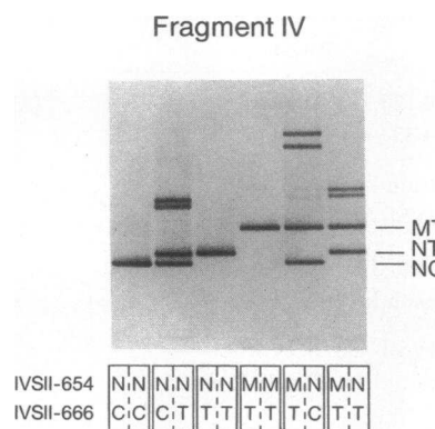
Figure 6. Gradient gel electrophoresis of fragment IV. The sequences of the normal C/T polymorphism at position 666 of the normal (N) or mutant (M) allele at position 654 are shown.
