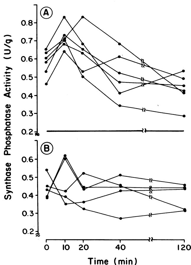
Figure 3. Individual synthase phosphatase activities at each time-point in group S (A) and group R (B).
