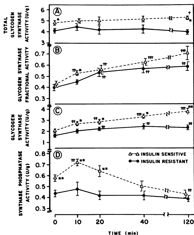
Figure 2. Change of total glycogen synthase activity (A); glycogen synthase fractional activity (B); active form of glycogen synthase activity (C); and synthase phosphatase activity (D) in group S ( \Delta ) and group R ( \bullet ). Glycogen synthase and synthase phosphatase activities were measured as described in Methods. Results are expressed as means±SE. T -test: * P < 0.05 , ** P < 0.01 between groups. Paired t -test: + P < 0.05 , ++ P < 0.01 , +++ P < 0.001 vs. 0 min.
